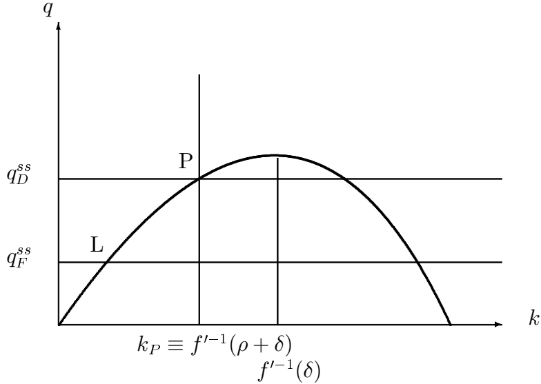
Figure 2: Steady state equilibrium under a quota
