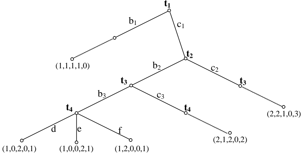
Figure 1: Payoffs
